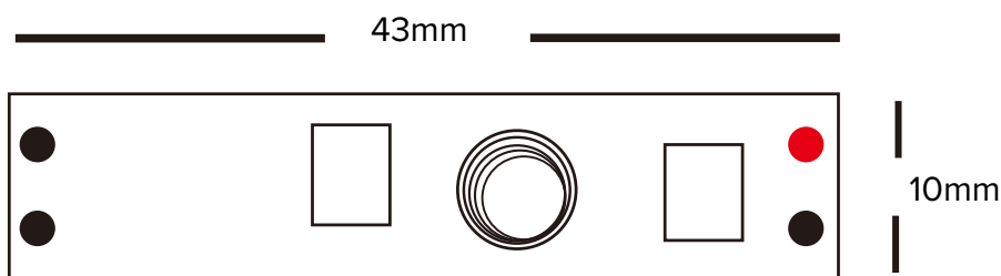
BS-PIR
